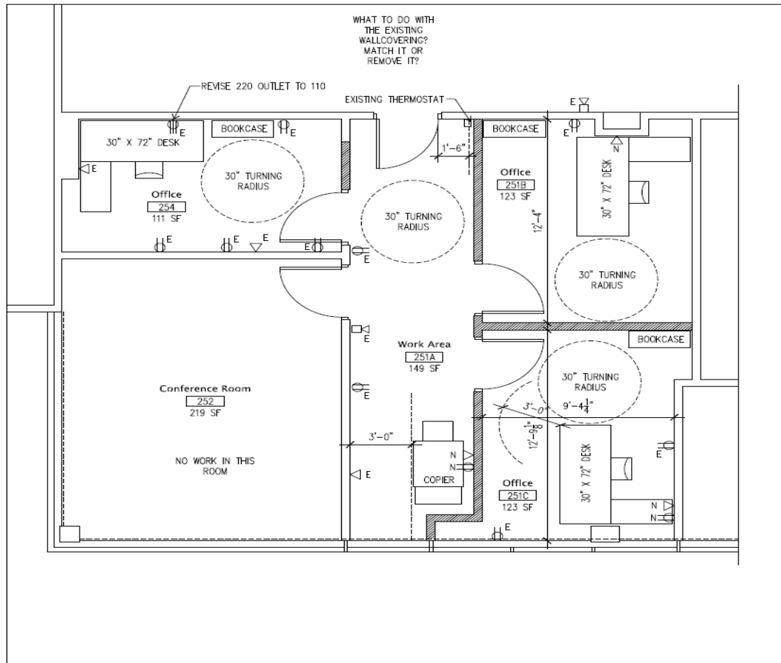
Floor Plan 1/4" = 1'-0"
